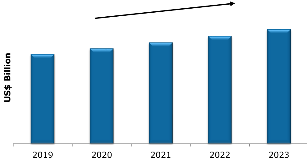
Global Heat Management Market by Value; 2019-2023 (US$ Billion)
