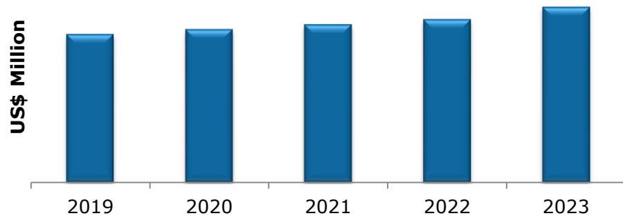
Global Desktop Cooling Fan Market by Value; 2019-2023 (US$ Million)
