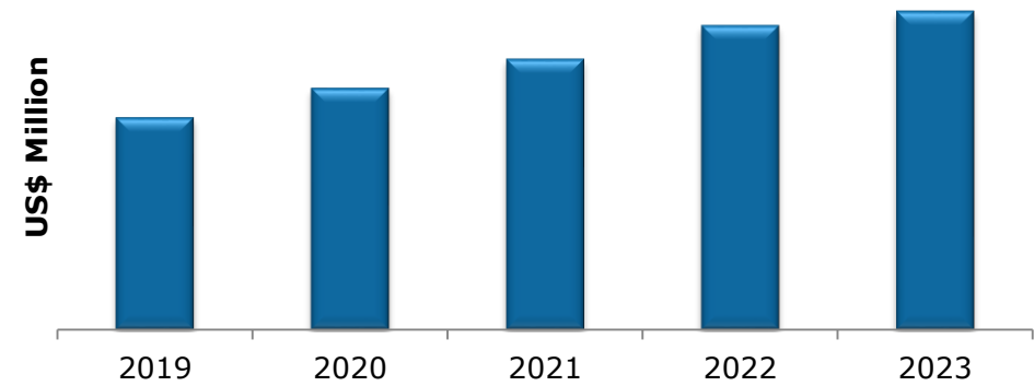
Global NB Cooling Fan Market by Value; 2019-2023 (US$ Million)
